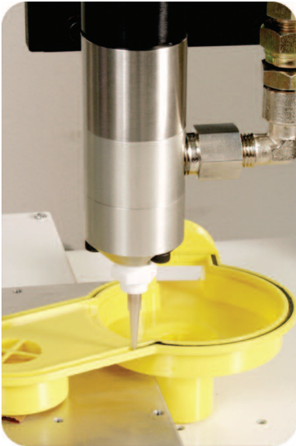
TS941 - gasketing.
